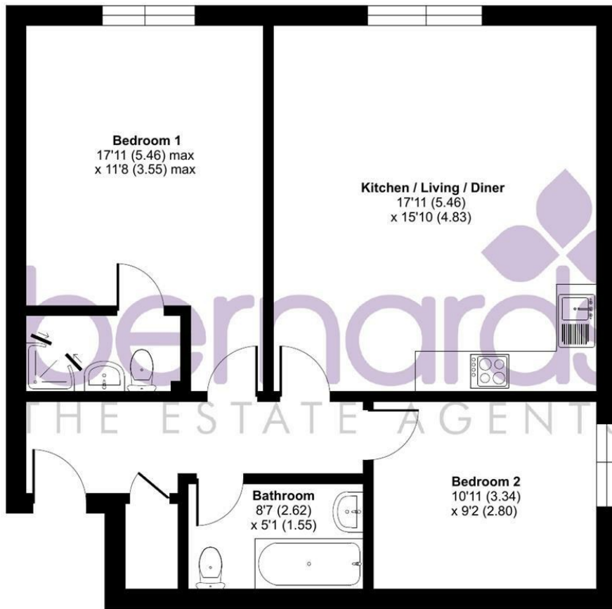
SECOND FLOOR
